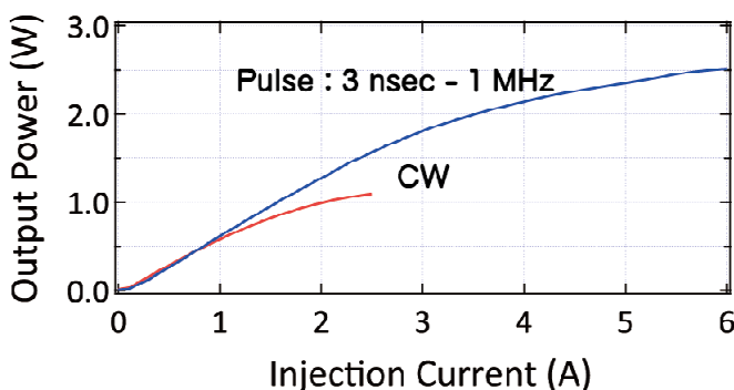
Output - Injection Current Properties
