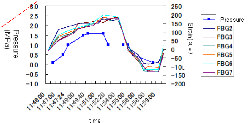
Linear strain movement along with pressure operation
